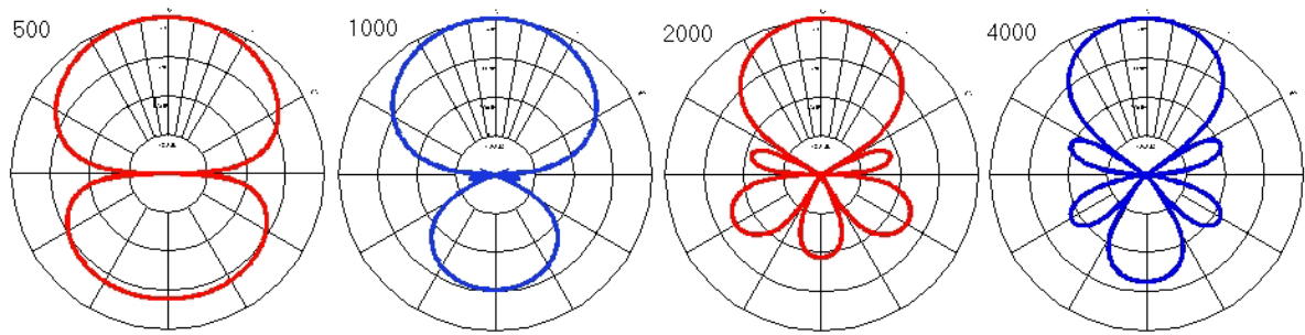
Fig. 4: Polar patterns of Endfire Array of 5 microphones, total length 10 cm.
