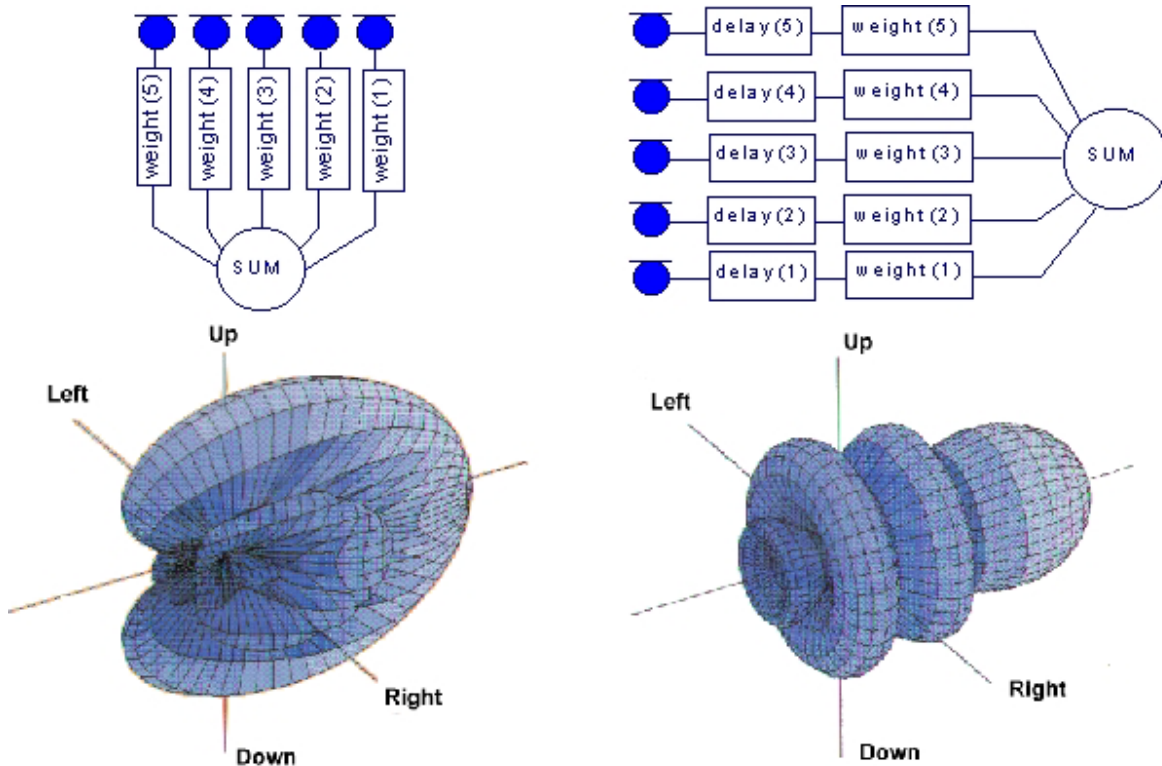
Fig. 1: Basic processing and 3D polar diagram of broadside array (left) and endfire array (right).
