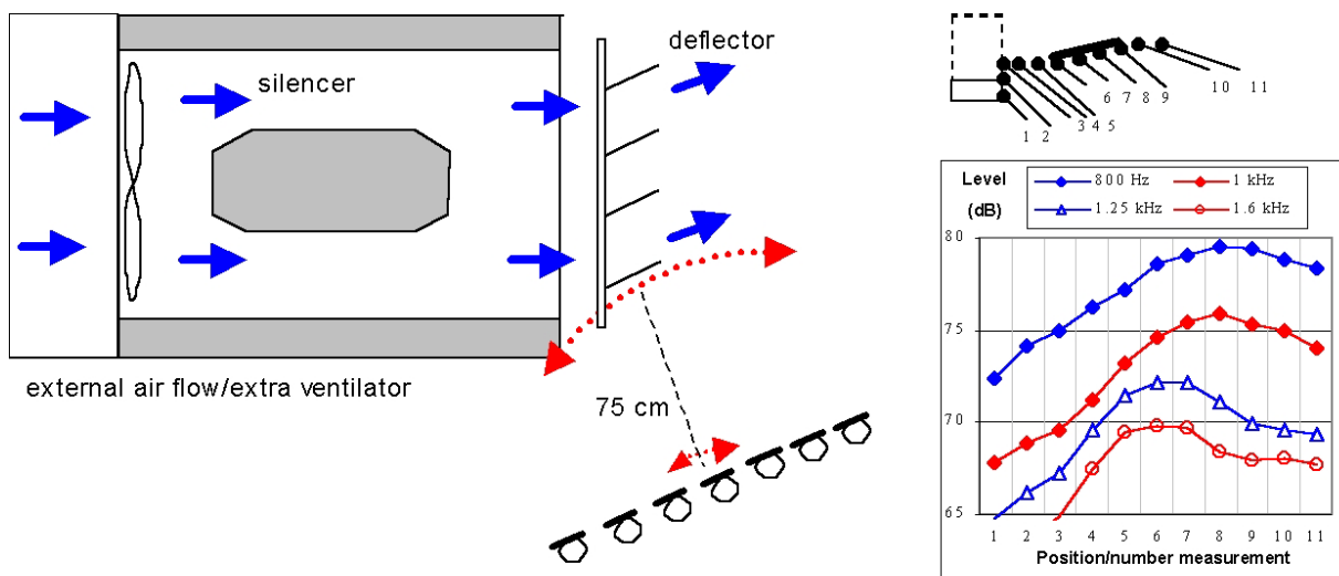
Fig. 3: Set-up (left) and typical result of tunnel ventilator with deflector blades (right).
