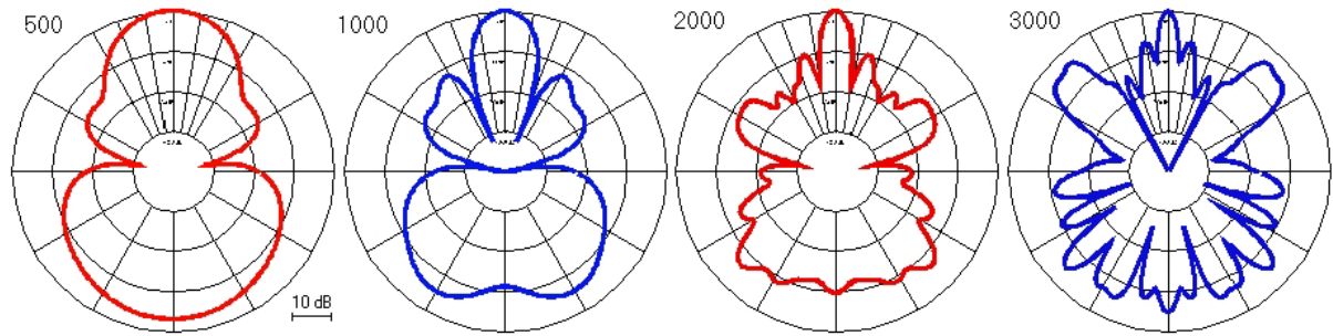
Fig. 2: Polar patterns of Broadside Array of 7 microphones, total width 80 cm.
