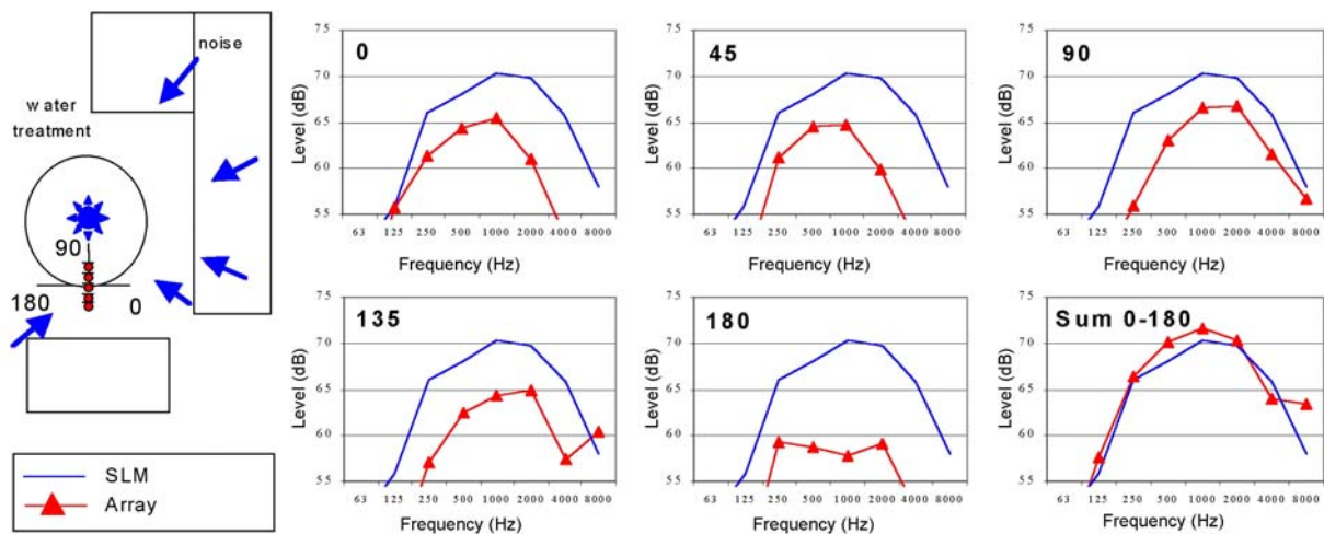
Fig. 5: Location of water treatment plant (left) and measurement results (right).
